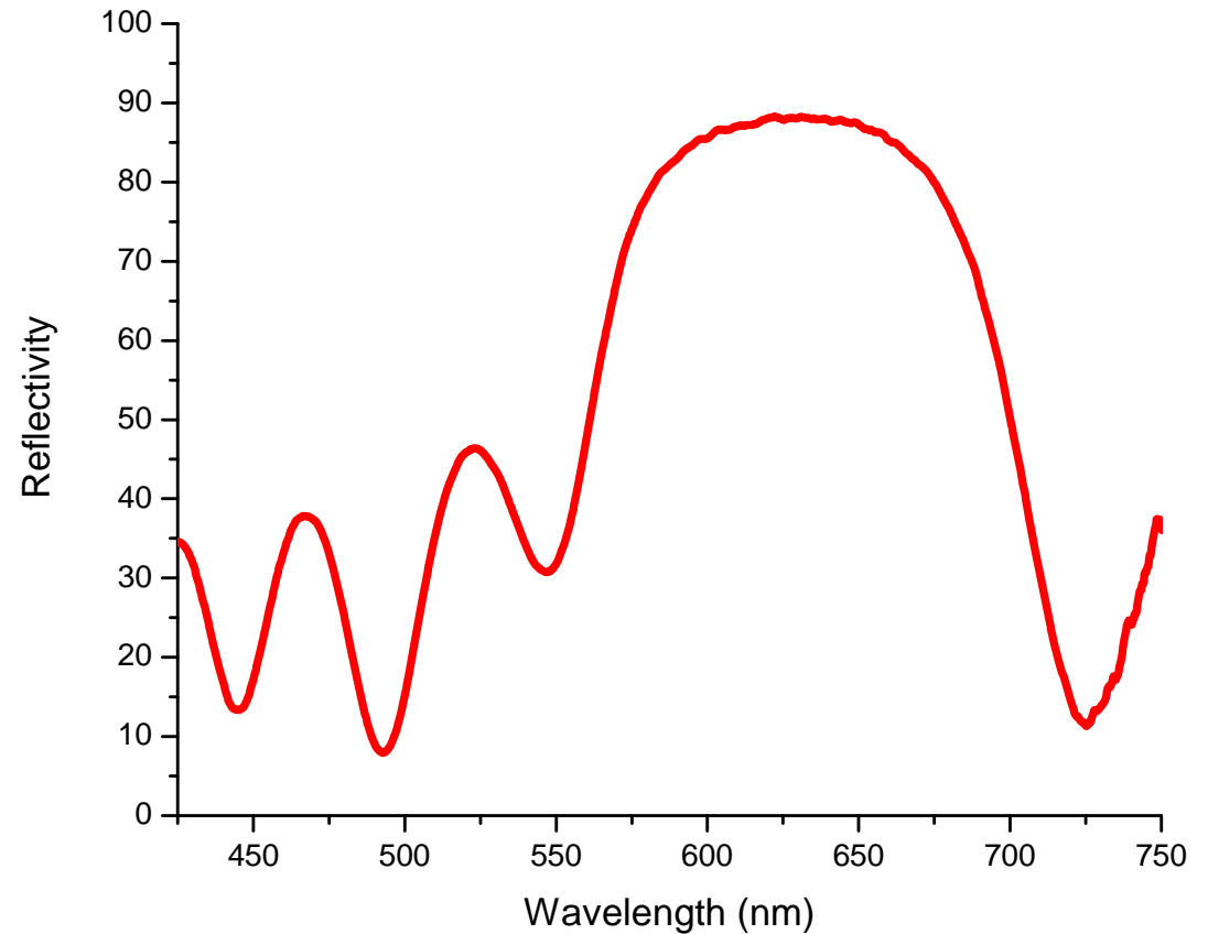
Reflectivity spectrum of a seven-period dielectric mirror composed of silica and titania mesoporous films as depicted in the schematic on left
