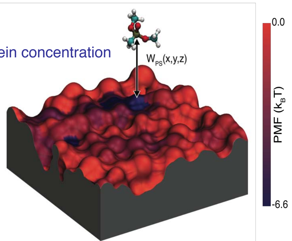
Small solute—Surface Interaction
