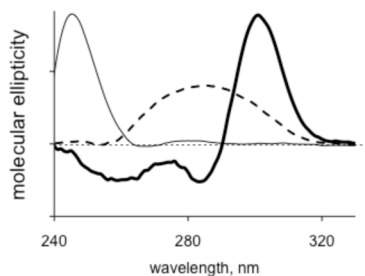
Figure 4. CD spectra of 1 in molecular ( \text{CH}_2\text{Cl}_2 – thin line, DMSO – dotted line) and ionic ( [\text{C}_4\text{-mim}]\text{BF}_4 – thick line) liquids.
