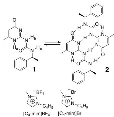
Scheme 2. Dimerization of 1 and some representative structures of ionic liquids.
