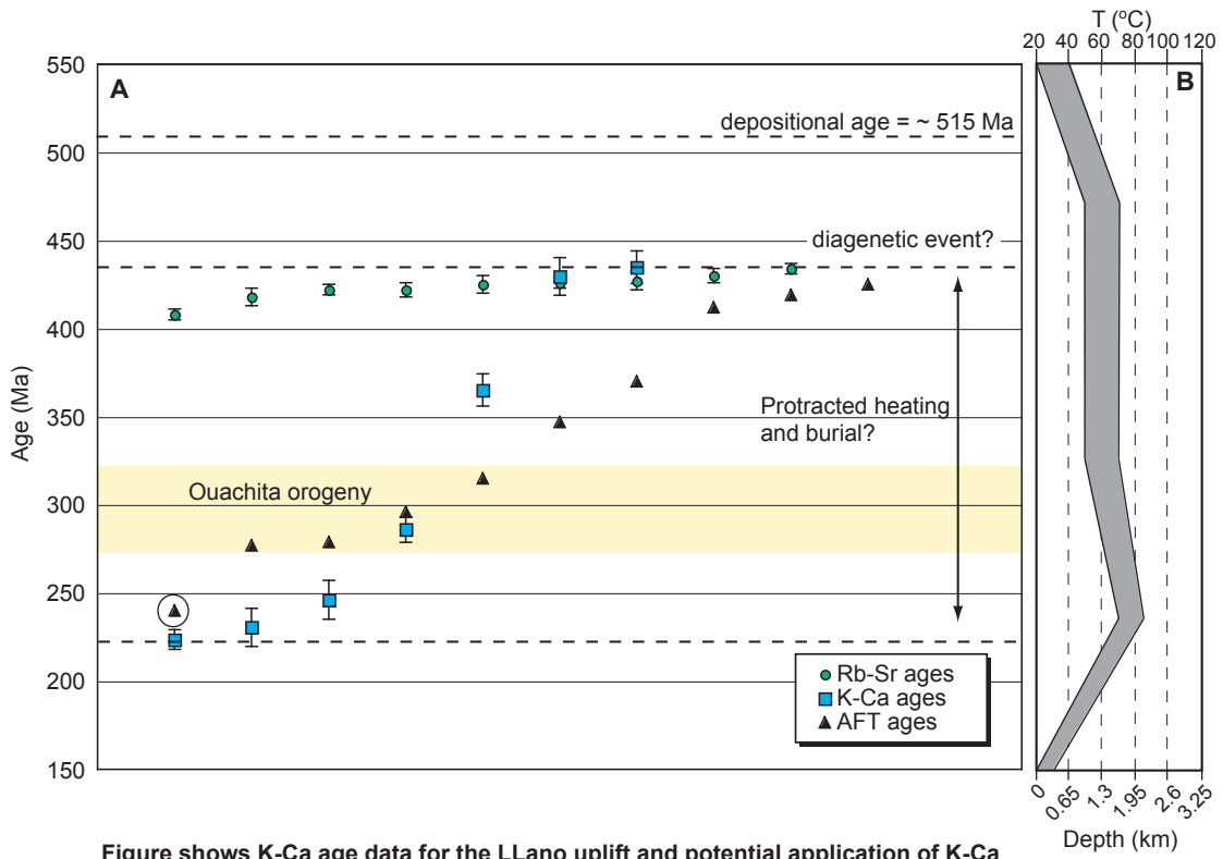
Figure shows K-Ca age data for the LLano uplift and potential application of K-Ca chronology as a low temperature thermochronometer.
