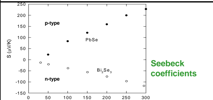
Nanostructured thermoelectric thin films
