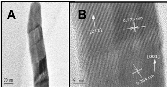
Heterostructured Bi 2 Se 3 nanowire with periodic interfaces between hexagonal and orthorhombic phases.
