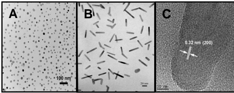
Spherical- and rod-shaped PbTe nanoparticles
