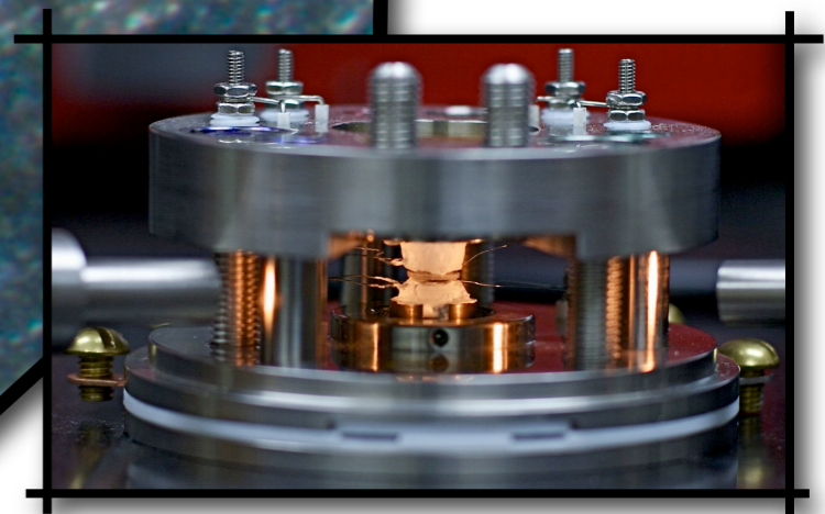
Hydrothermal Diamond Anvil Cell
