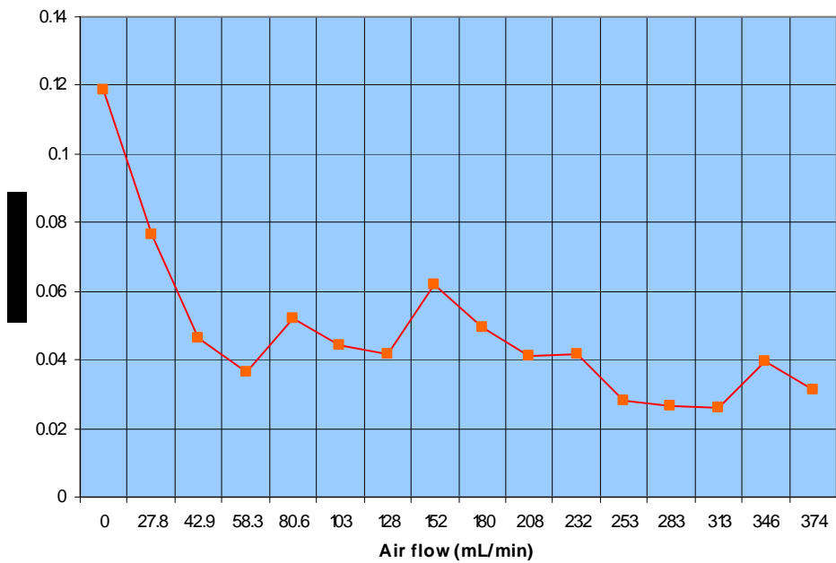
Figure 4. Air flow versus emission intensity at a steady power of 75 W.
