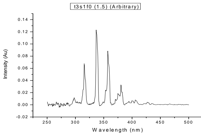
Figure 3. Optical emission spectra of CPE.
