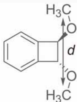
trans benzocyclobutene
