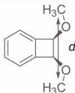
cis benzocyclobutene
