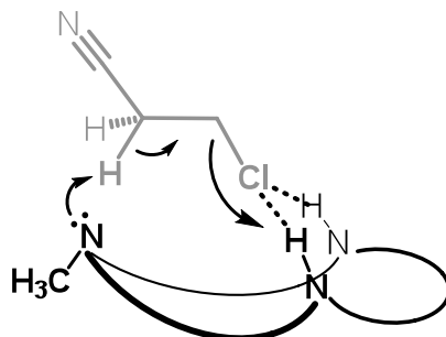
Prereaction complex showing syn orientation of electrophile
