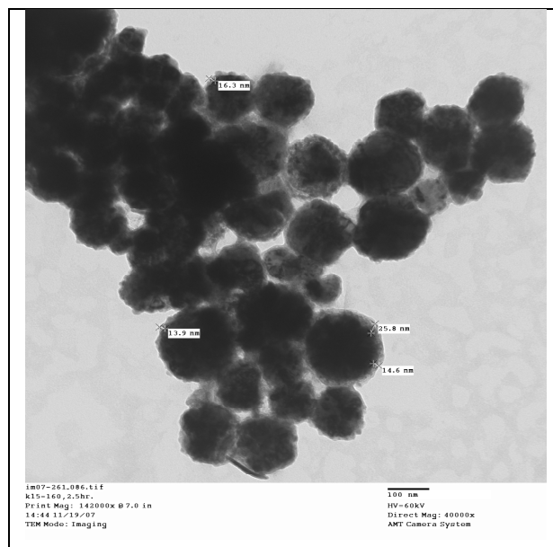
Figure 4: FeNi nanoparticles coated with amorphous carbon synthesized using “Green” synthesis technique.
