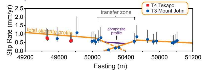
D. Slip Rate Profile
