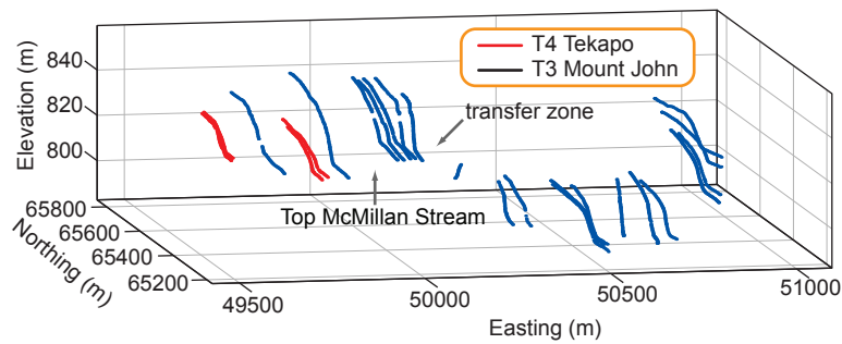
B. Fault Scarp Profiles
