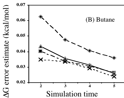
Error estimates for solvation free energy calculations of methane (A) and butane (B) in water, comparing conventional molecular dynamics ( \diamond ), WHAM ( \square ), REMD ( \triangle ), and REMD plus WHAM (X).
