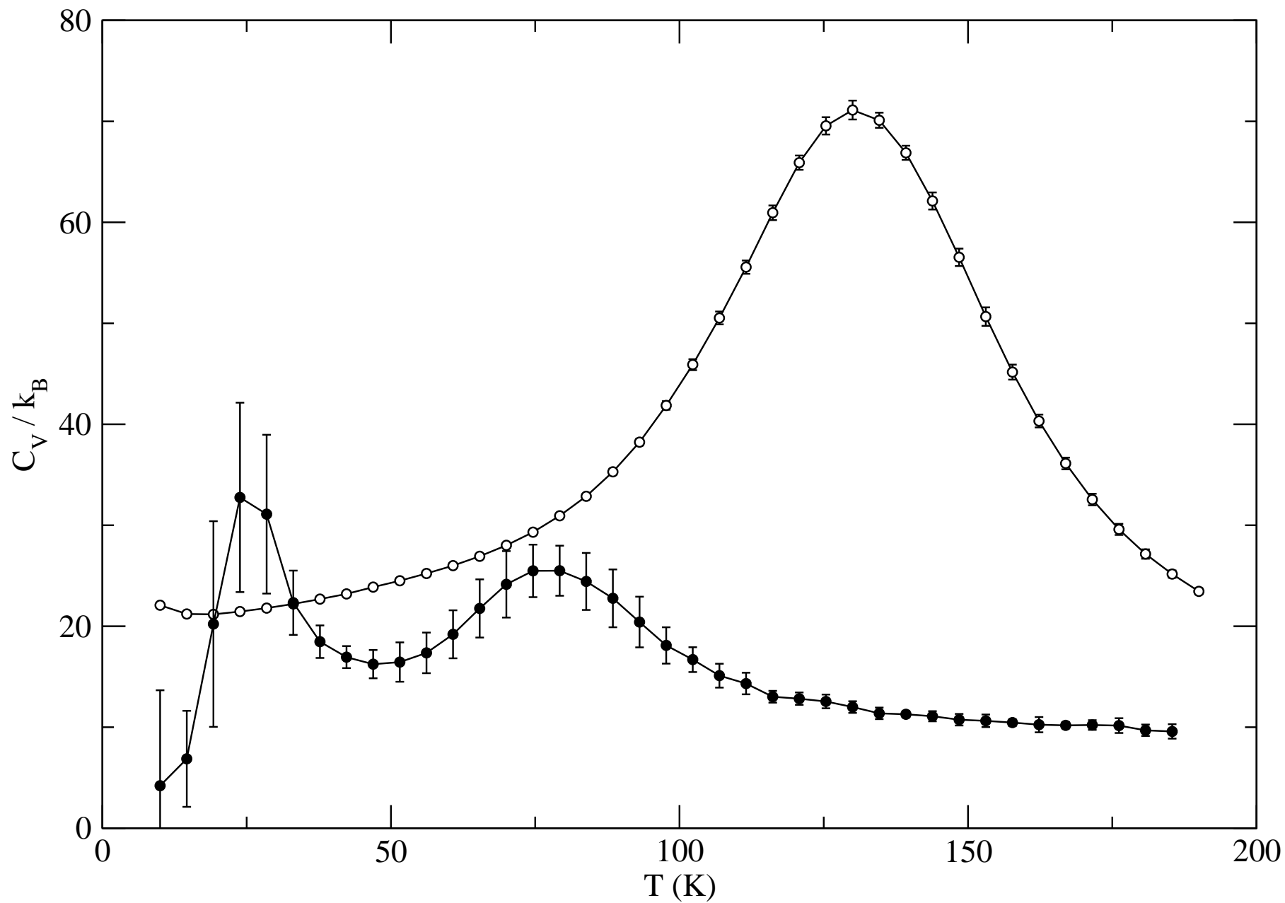
The classical (white circles) and quantum (black circles) heat capacity of (\text{HCL})_5
